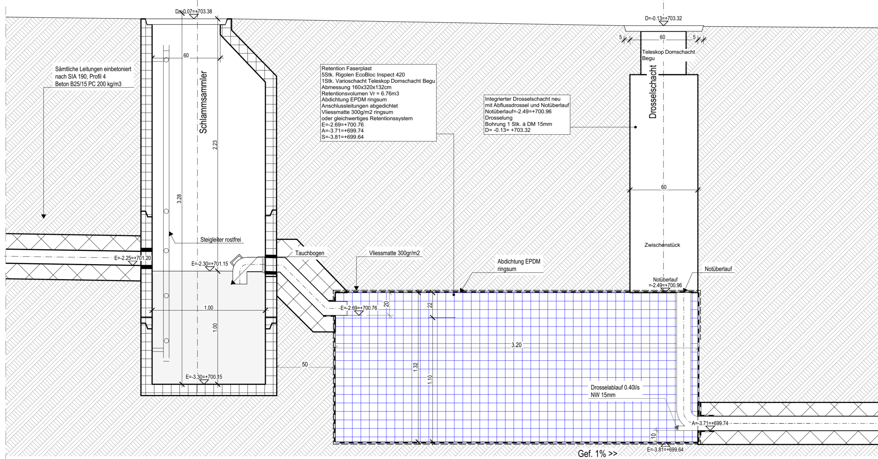
Detail EG Retention, 1:20
